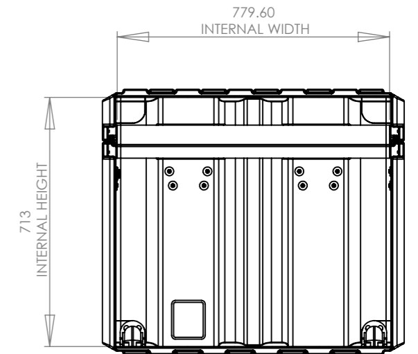
SECTION Z-Z SCALE 1 : 15
