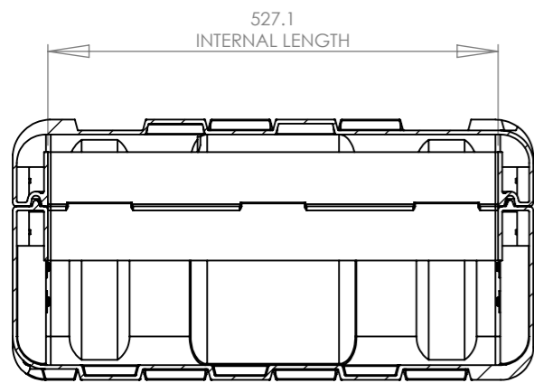
SECTION Y-Y
