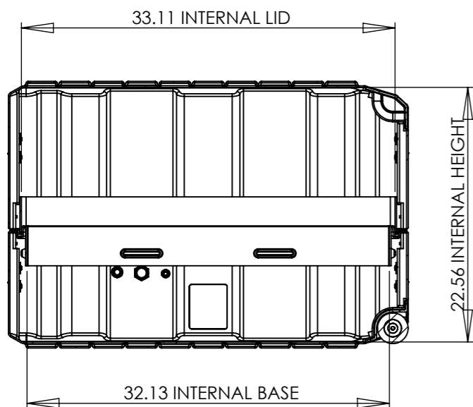
SECTION Y-Y SCALE 1 : 12
