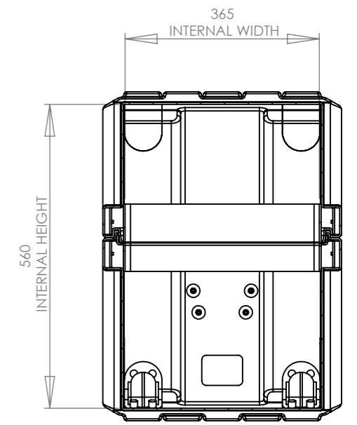
SECTION Z-Z
